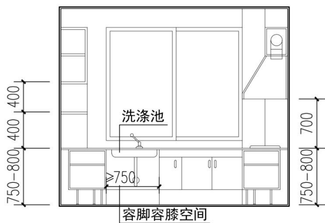
(c) 2-2 剖面图
